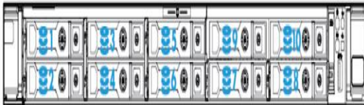
1-10 10 x SFF SATA/SAS/SSD Hot Pluggable Hard Drive Bays
